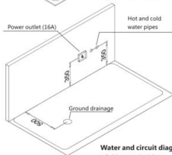
Water and circuit diagram of skirts on 4 sides
